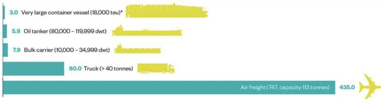
Figure 1: Comparison of typical CO 2 emissions between modes of transport, in grams/tonne-km 2
